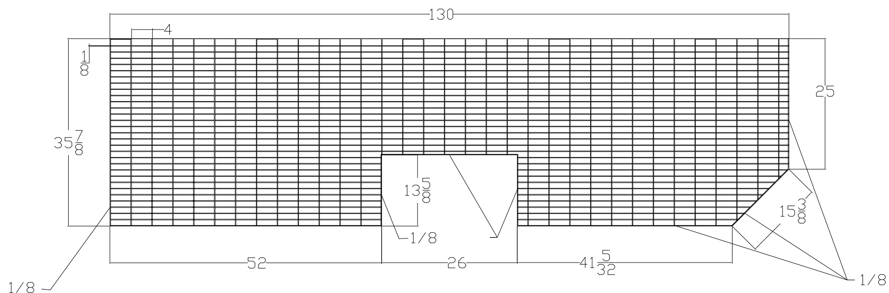
Floor Grate 2 Mat'l-1" 19W4 Floor Grating Serrated
