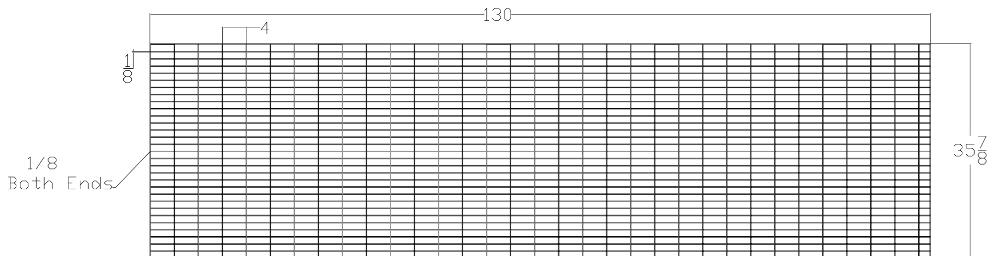
Floor Grate 1 Mat'l-1" 19W4 Floor Grating Serrated
